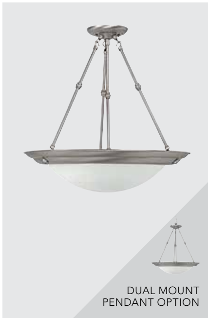
▲ 2720MN PENDANT Matte Nickel 20"W x 20.75"H Maximum Hanging Height: 98.75" 72" Chain; 120" Wire Canopy: 5"W x 1"H 3 - 100 Watt E26 Medium White Faux Alabaster Glass Convertible Dual Mount
