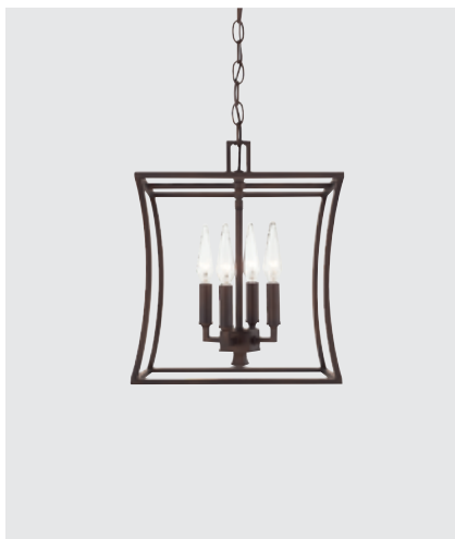
WESTBROOK ◀ 510141WG FOYER Winter Gold ◀ 510141BB FOYER Burnished Bronze 12"W x 14.75"H Maximum Hanging Height: 140.75" 120" Chain; 180" Wire Canopy: 5"W x 0.75"H 4 - 60 Watt E12 Candelabra
