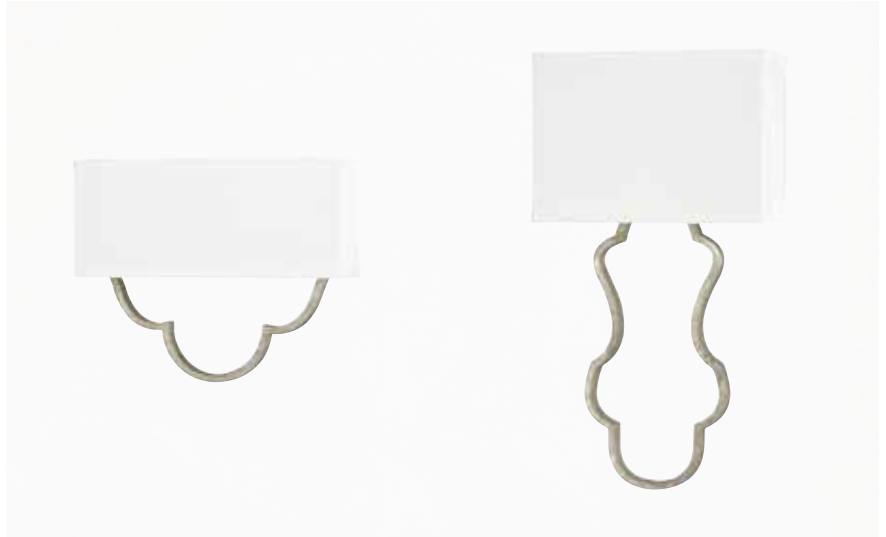
▲ 4942AS-636 SCNCE Antique Silver 12.50"W x 10.50"H x 4.25"E Backplate: 12.50"W x 5.50"H x 1.25"E Ctr/Top: 2.75" Ctr/Btm: 7.75" 2 - 60 Watt E12 Candelabra White Fabric Stay-Straight Shade Damp Rated
