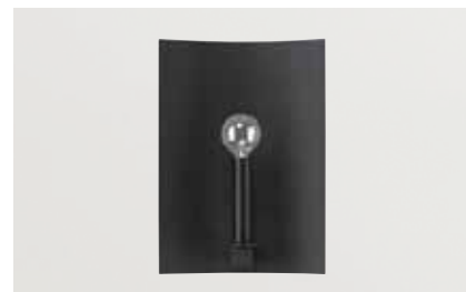
▶ 4911BI SCONCE Black Iron 8.25"W x 11.75"H x 3.25"E Backplate: 4.50"W x 11"H x 0.75"E Ctr/Top: 6" Ctr/Btm: 5.75" 1 - 60 Watt E12 Candelabra Damp Rated ADA
